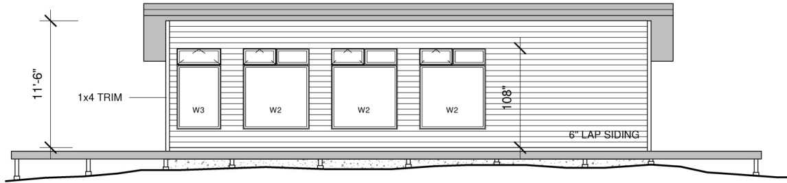
FRONT ELEVATION
