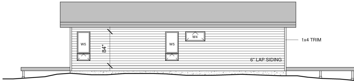
REAR ELEVATION
